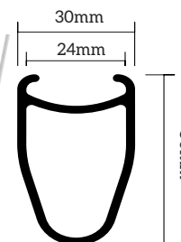
SYMMETRIC 622 x 24C
