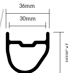
ASYMMETRIC HOOKLESS 622 x 30C
