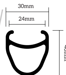
HOOKLESS SYMMETRIC 622 x 24C
