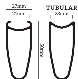
RIM Detail
