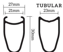
RIM Detail
