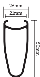
RIM Detail
