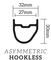
RIM Detail
