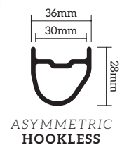
RIM Detail
