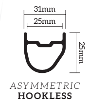
RIM Detail
