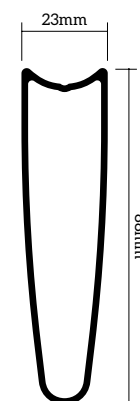
RIM Detail
