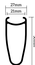
RIM Detail
