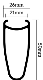
RIM Detail
