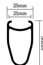
RIM Detail
