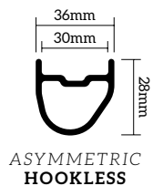
RIM Detail
